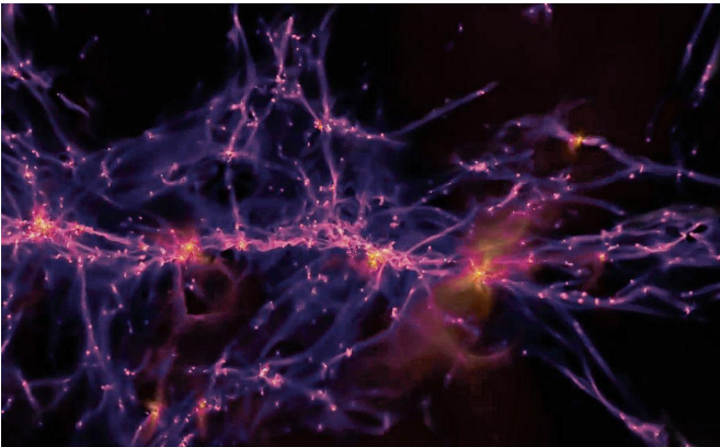
Simulation of star clustering. Gas filaments in purple. Light emission in yellow. Curtesy Henry Katz / SPHINX Collaboration
